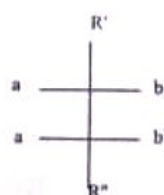
erythro form
