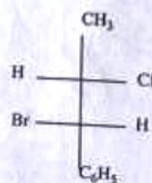
threo form
