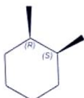
Cis isomer
