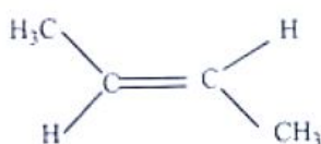
Trans isomer
