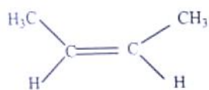
Cis isomer
