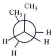
Eclipsed
