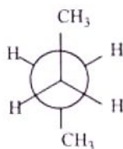
Anti
