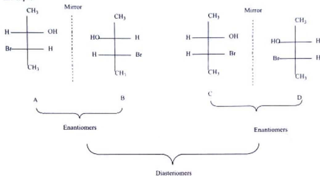
Four isomers of 3-Bromo-2-butanol
