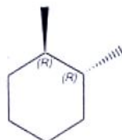
Trans isomer
