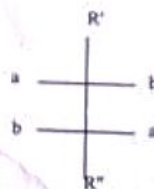
threo form
