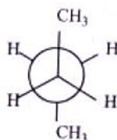
Anti
