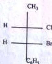
erythro form
