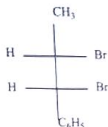
erythro form
