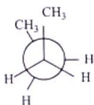
Eclipsed
