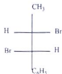
threo form
